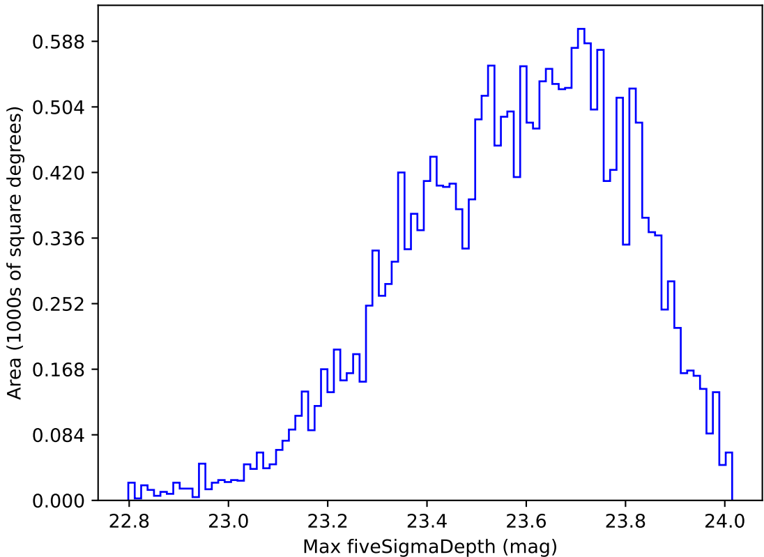
extra_ss_neo2_v3.4_10yrs Yr 1 u band: Max fiveSigmaDepth
