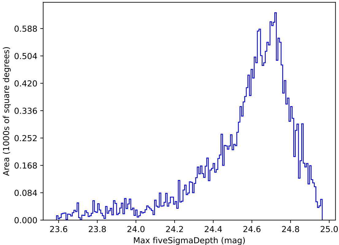
extra_ss_neo2_v3.4_10yrs Yr 1 r band: Max fiveSigmaDepth
