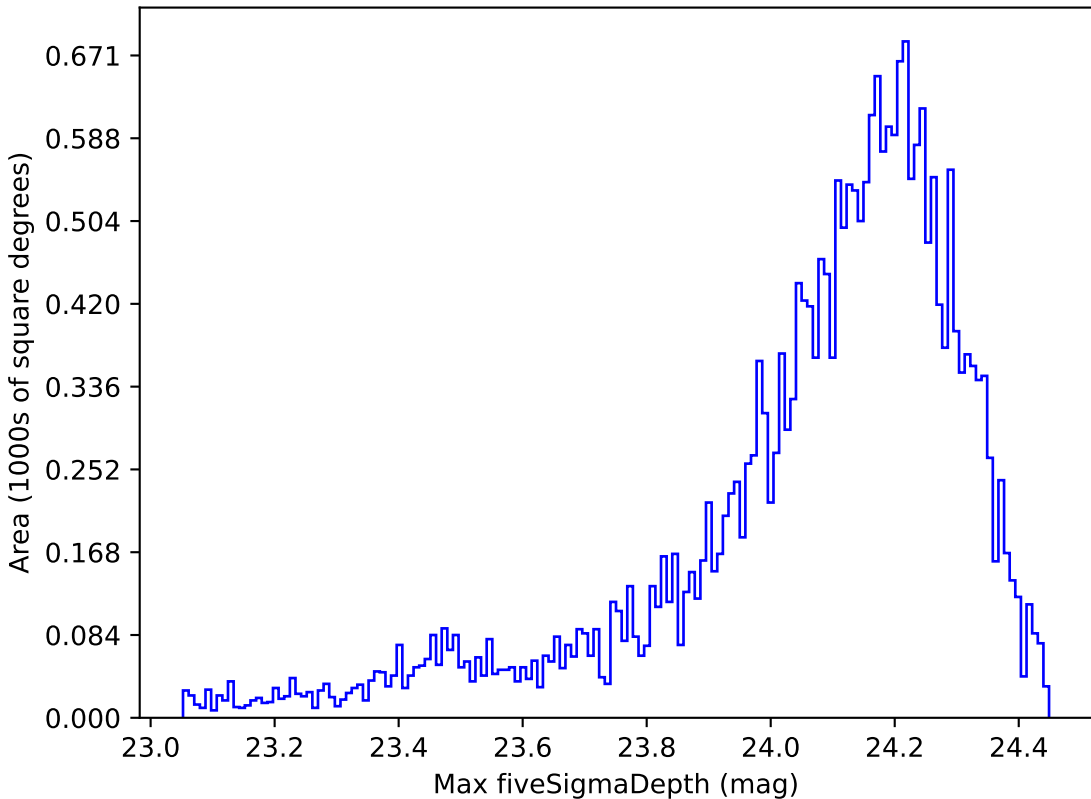
extra_ss_neo2_v3.4_10yrs Yr 1 i band: Max fiveSigmaDepth
