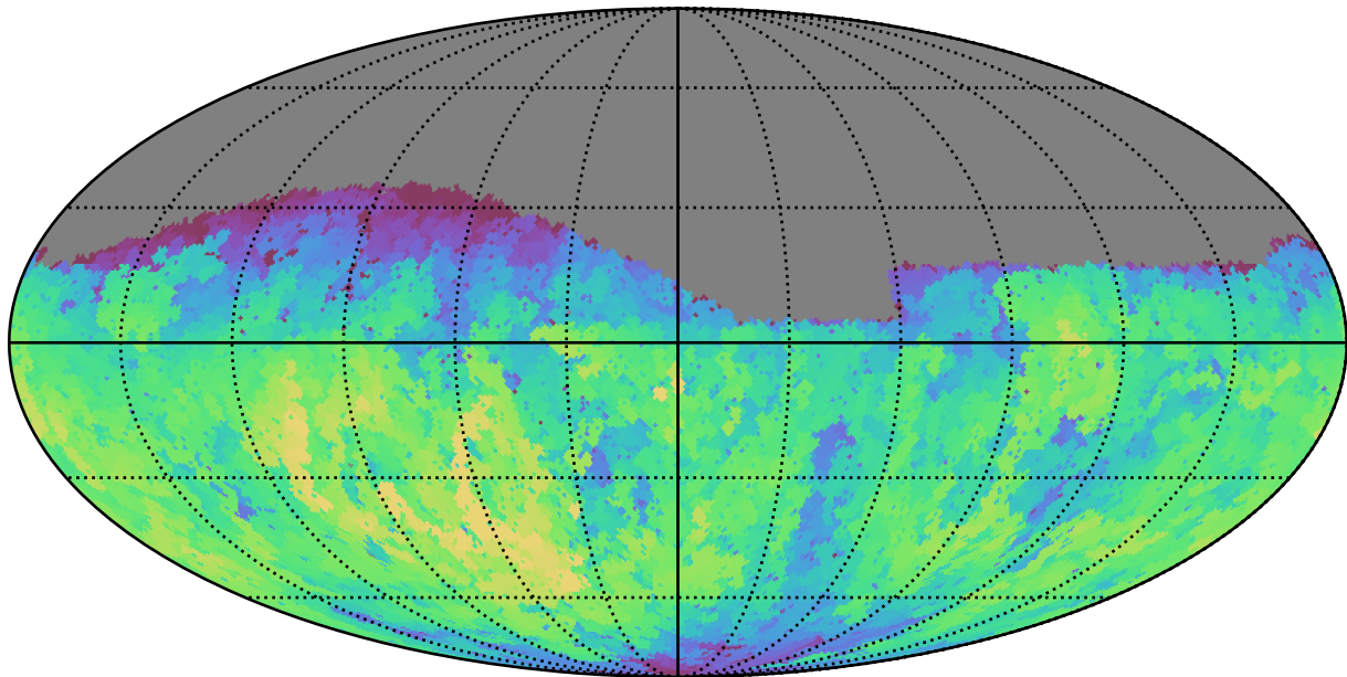
extra_ss_neo2_v3.4_10yrs Yr 1 g band: Max fiveSigmaDepth
