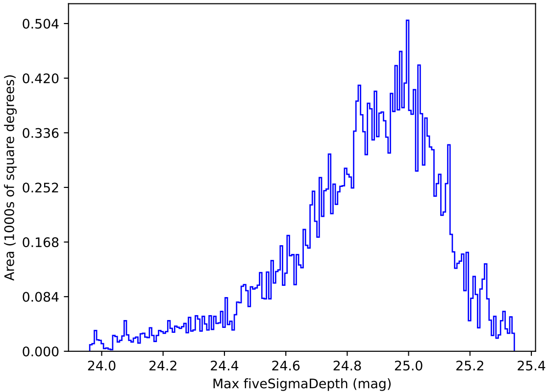
extra_ss_neo2_v3.4_10yrs Yr 1 g band: Max fiveSigmaDepth
