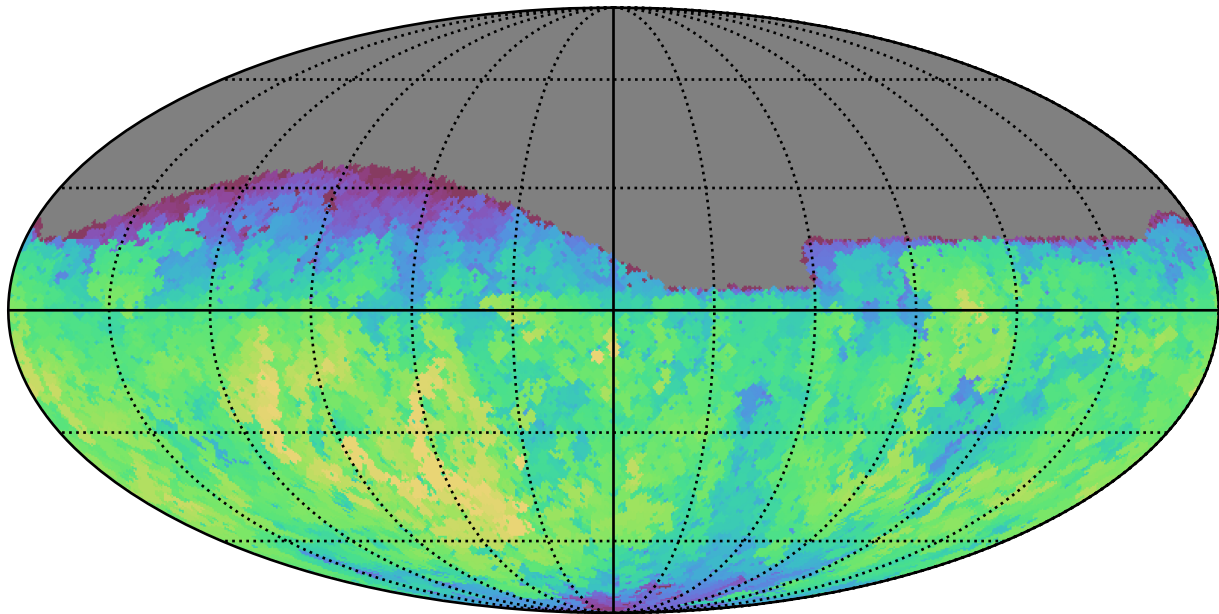
extra_ss_neo2_v3.4_10yrs Yr 1 all bands: Max fiveSigmaDepth
