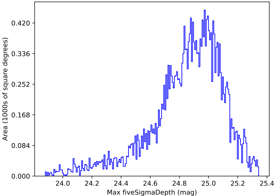
extra_ss_neo2_v3.4_10yrs Yr 1 all bands: Max fiveSigmaDepth
