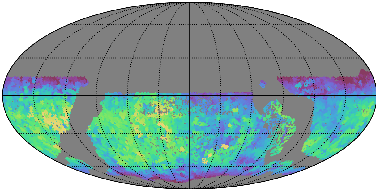
extra_ss_neo2_v3.4_10yrs WFD z band: Max fiveSigmaDepth
