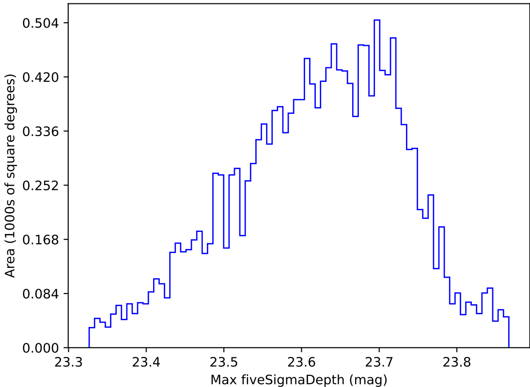
extra_ss_neo2_v3.4_10yrs WFD z band: Max fiveSigmaDepth
