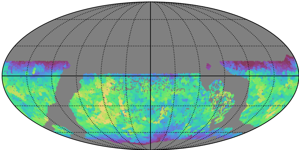
extra_ss_neo2_v3.4_10yrs WFD y band: Max fiveSigmaDepth
