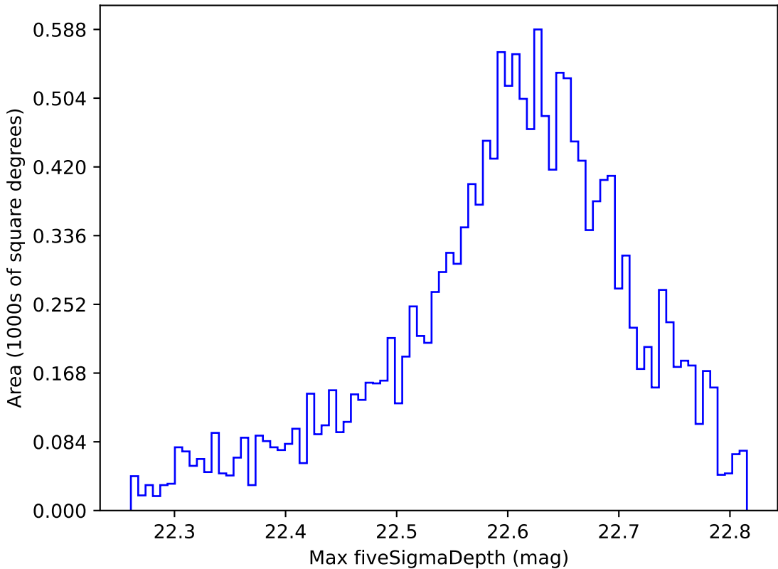
extra_ss_neo2_v3.4_10yrs WFD y band: Max fiveSigmaDepth
