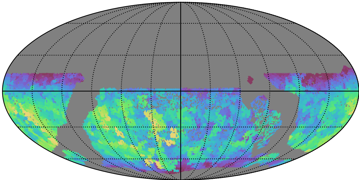
extra_ss_neo2_v3.4_10yrs WFD u band: Max fiveSigmaDepth
