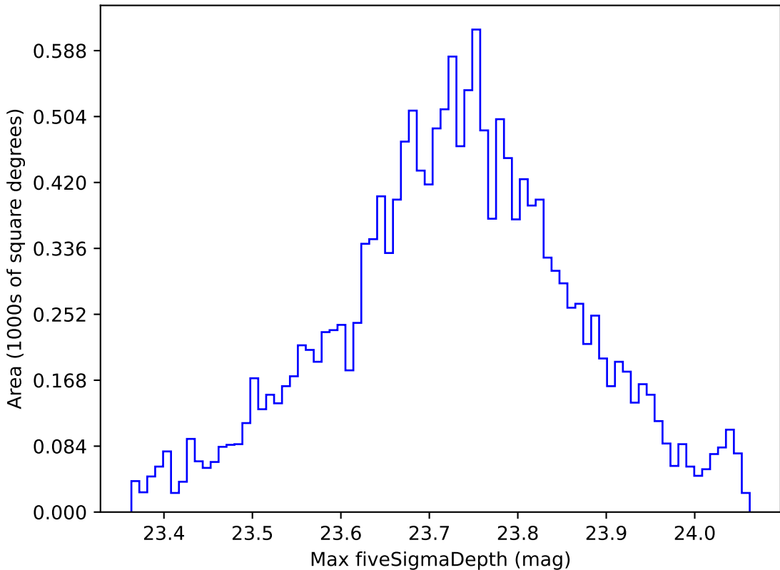
extra_ss_neo2_v3.4_10yrs WFD u band: Max fiveSigmaDepth
