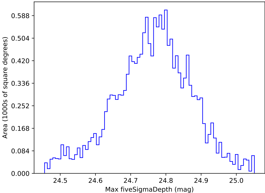
extra_ss_neo2_v3.4_10yrs WFD r band: Max fiveSigmaDepth
