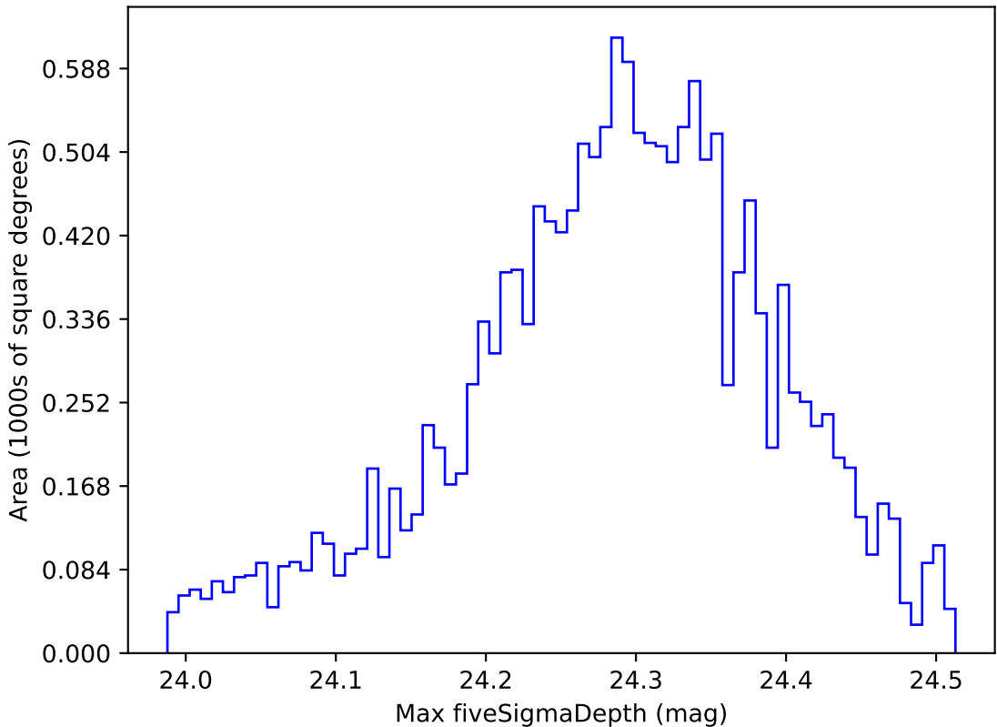
extra_ss_neo2_v3.4_10yrs WFD i band: Max fiveSigmaDepth
