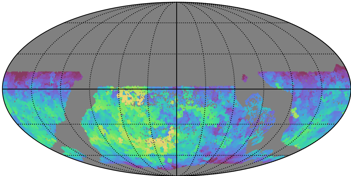
extra_ss_neo2_v3.4_10yrs WFD g band: Max fiveSigmaDepth
