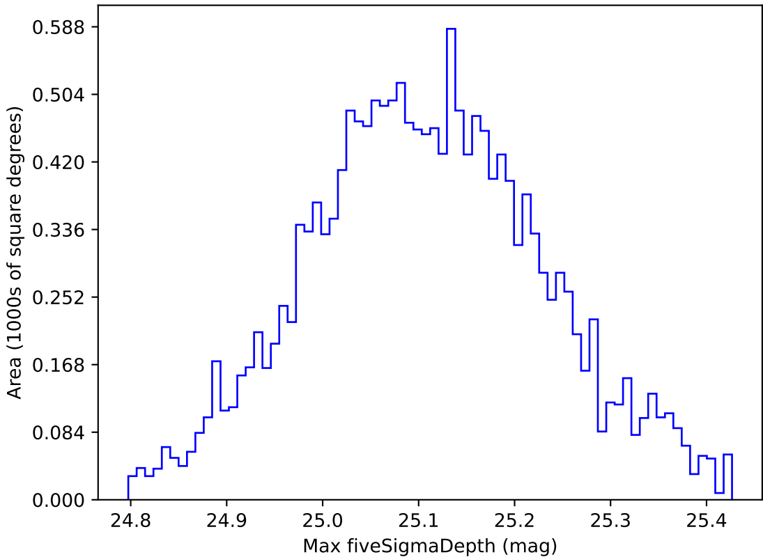
extra_ss_neo2_v3.4_10yrs WFD g band: Max fiveSigmaDepth
