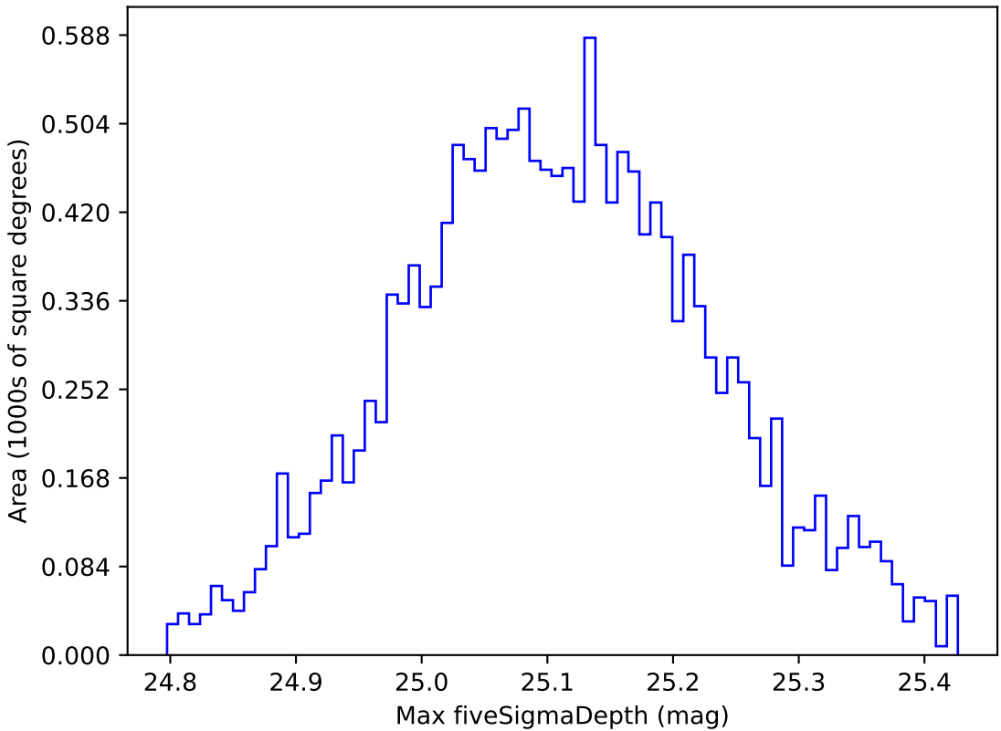
extra_ss_neo2_v3.4_10yrs WFD all bands: Max fiveSigmaDepth
