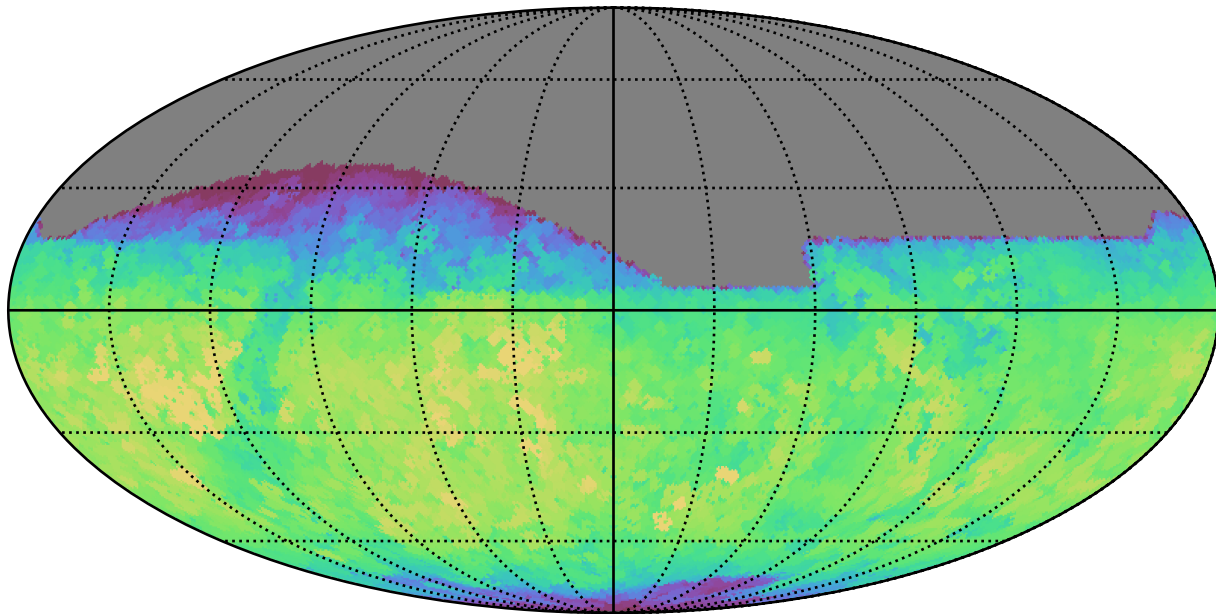
extra_ss_neo2_v3.4_10yrs All sky z band: Max fiveSigmaDepth
