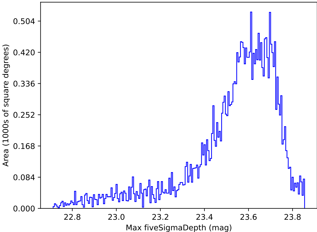
extra_ss_neo2_v3.4_10yrs All sky z band: Max fiveSigmaDepth
