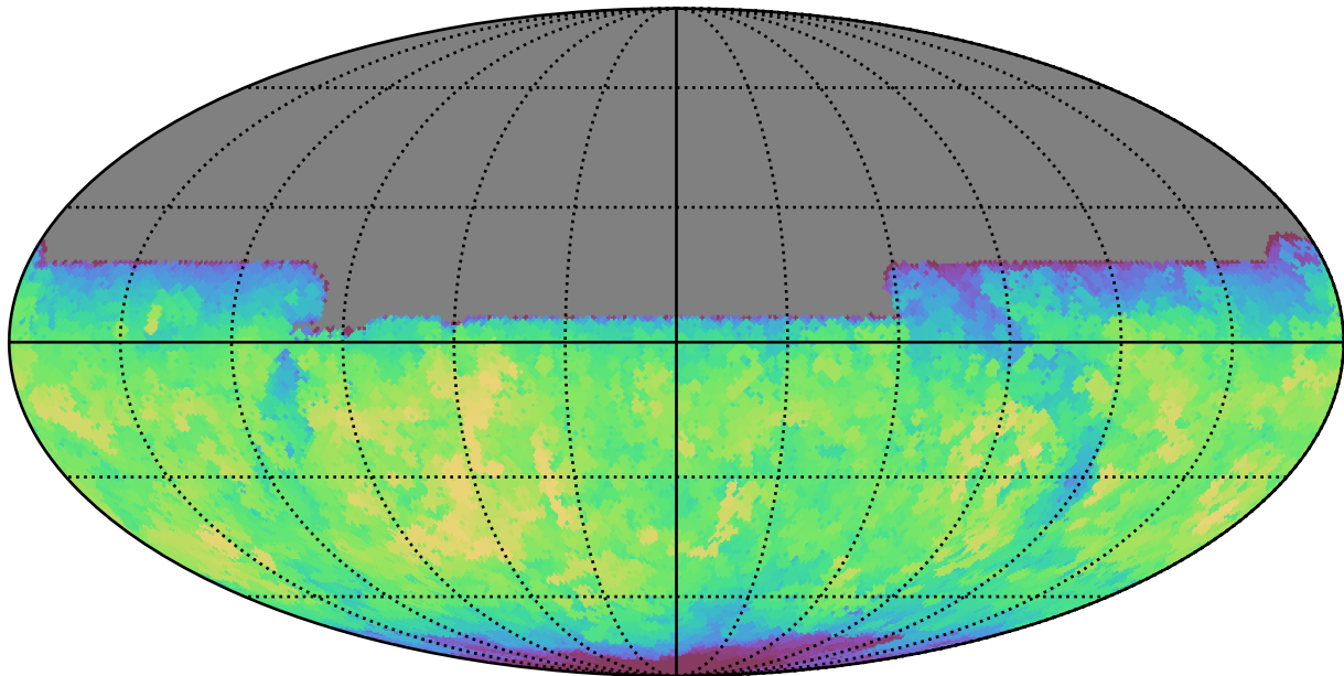
extra_ss_neo2_v3.4_10yrs All sky y band: Max fiveSigmaDepth
