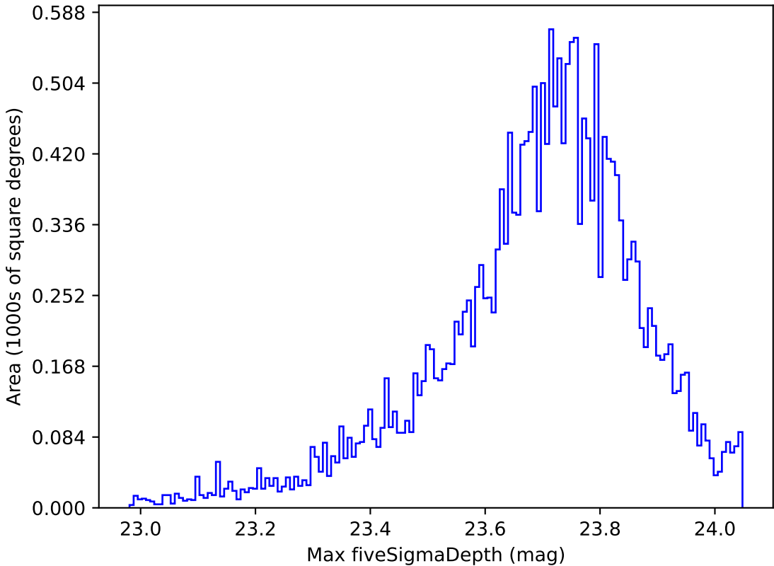
extra_ss_neo2_v3.4_10yrs All sky u band: Max fiveSigmaDepth
