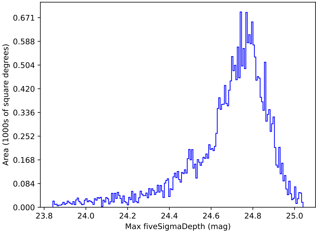
extra_ss_neo2_v3.4_10yrs All sky r band: Max fiveSigmaDepth
