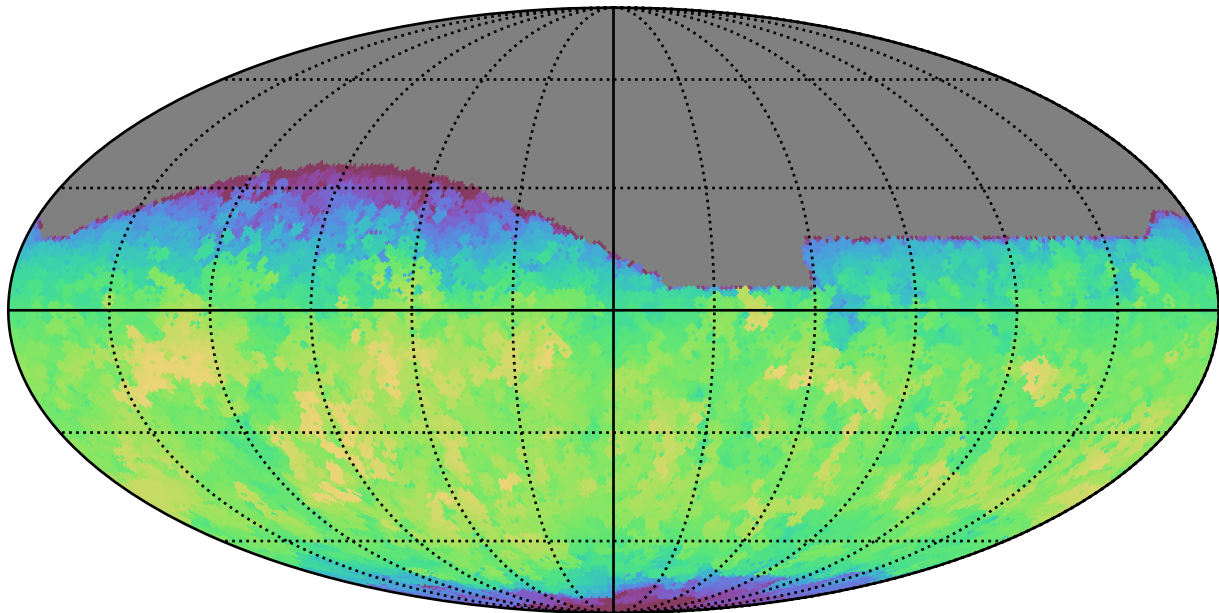
extra_ss_neo2_v3.4_10yrs All sky i band: Max fiveSigmaDepth
