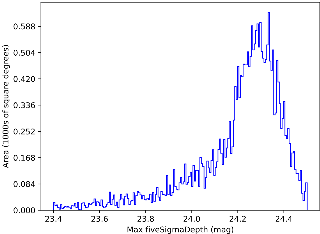
extra_ss_neo2_v3.4_10yrs All sky i band: Max fiveSigmaDepth
