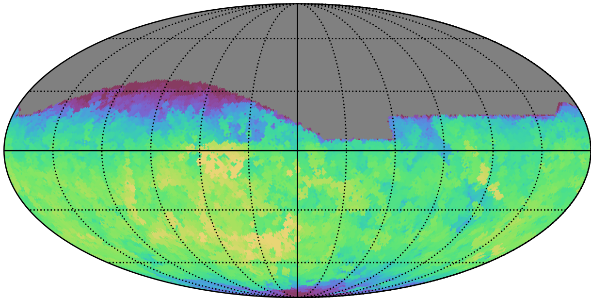
extra_ss_neo2_v3.4_10yrs All sky g band: Max fiveSigmaDepth
