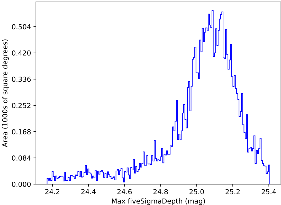
extra_ss_neo2_v3.4_10yrs All sky g band: Max fiveSigmaDepth
