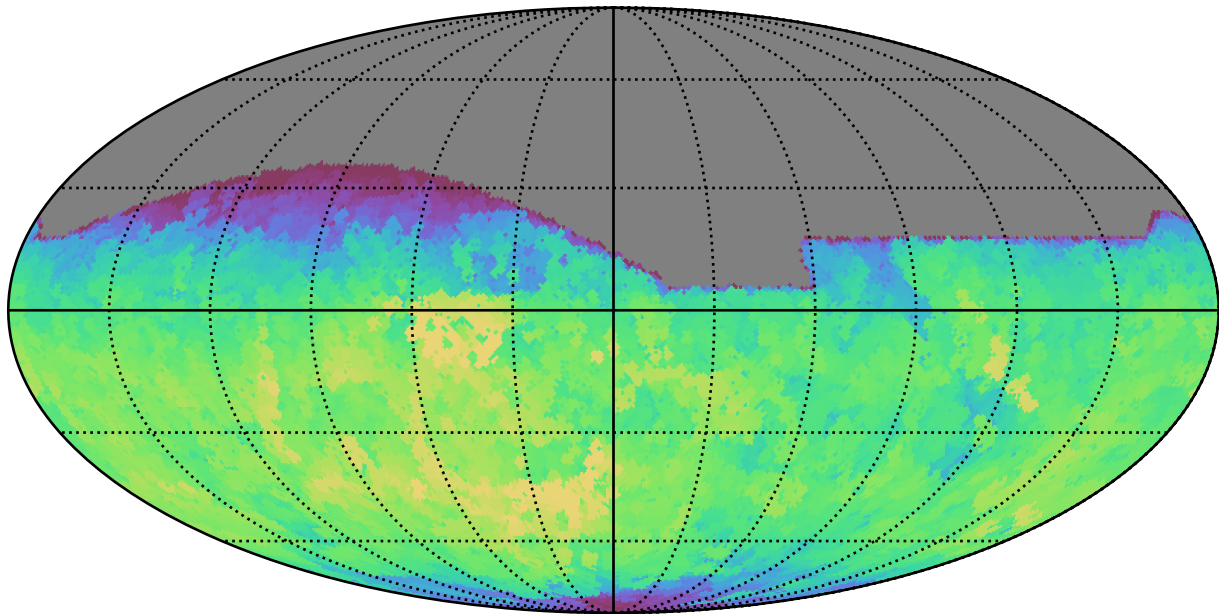
extra_ss_neo2_v3.4_10yrs All sky all bands: Max fiveSigmaDepth
