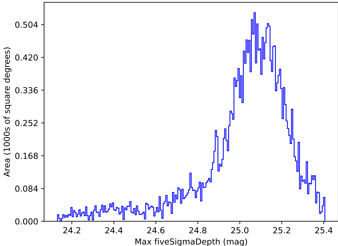
extra_ss_neo2_v3.4_10yrs All sky all bands: Max fiveSigmaDepth
