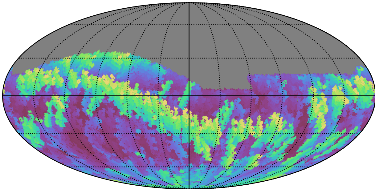
extra_ss_neo2_v3.4_10yrs Yr 1 z band: Max airmass
