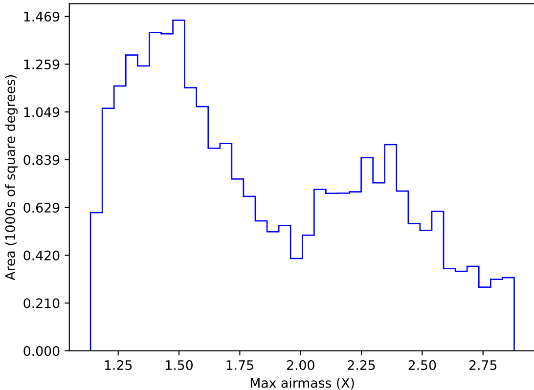
extra_ss_neo2_v3.4_10yrs Yr 1 z band: Max airmass
