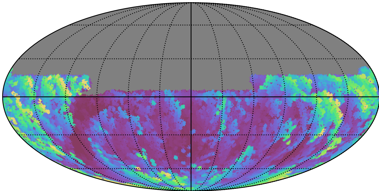
extra_ss_neo2_v3.4_10yrs Yr 1 y band: Max airmass
