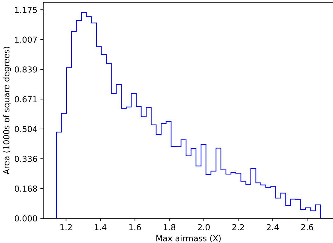
extra_ss_neo2_v3.4_10yrs Yr 1 y band: Max airmass
