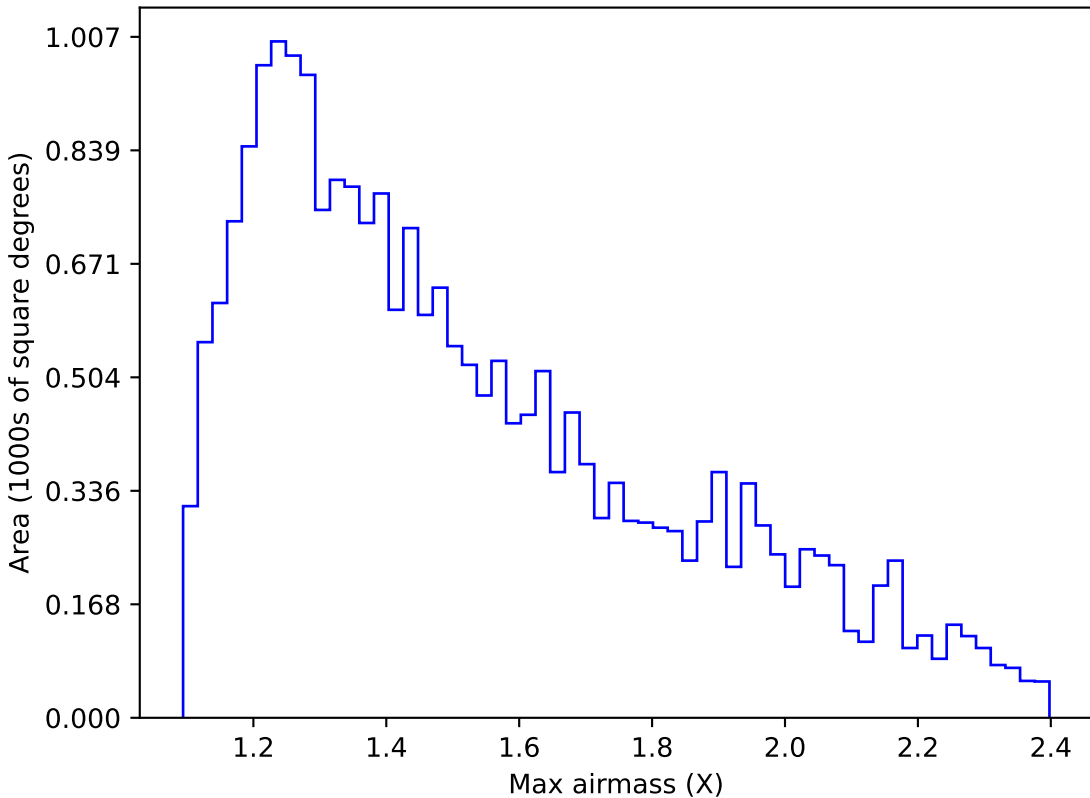
extra_ss_neo2_v3.4_10yrs Yr 1 u band: Max airmass
