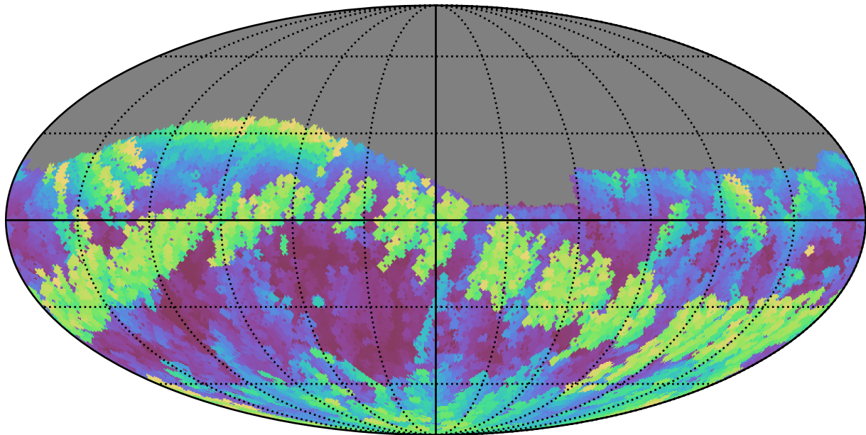
extra_ss_neo2_v3.4_10yrs Yr 1 r band: Max airmass
