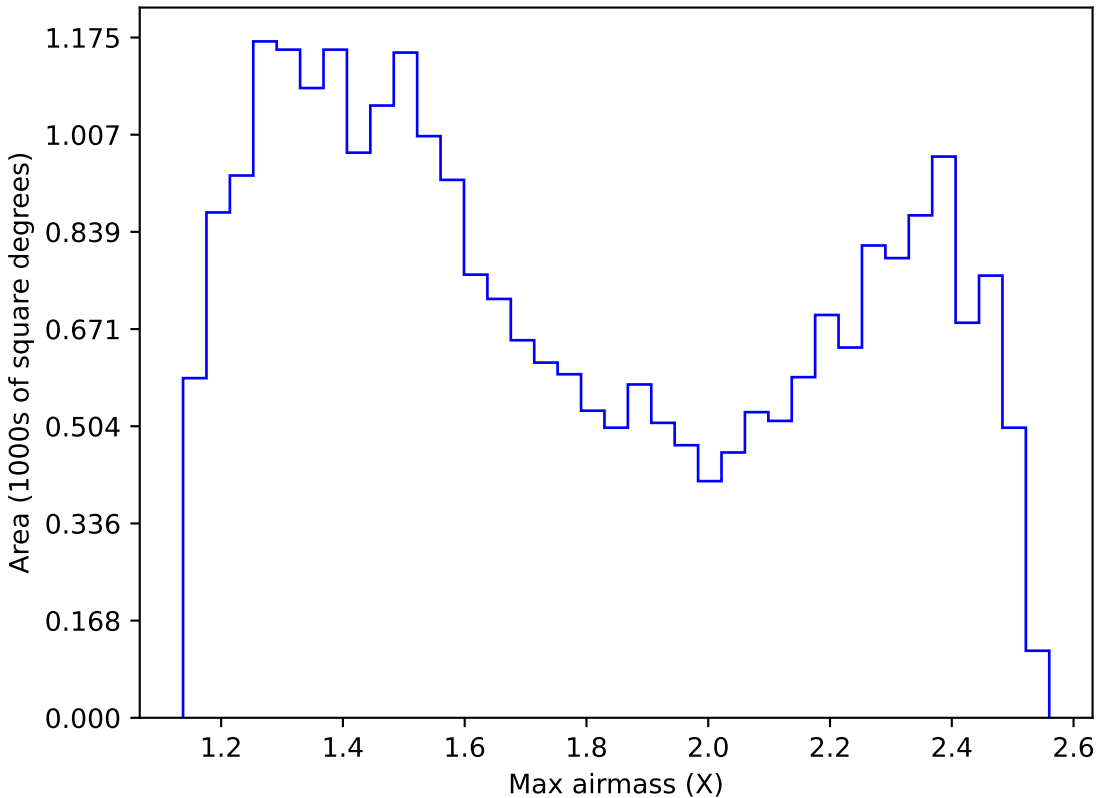
extra_ss_neo2_v3.4_10yrs Yr 1 r band: Max airmass
