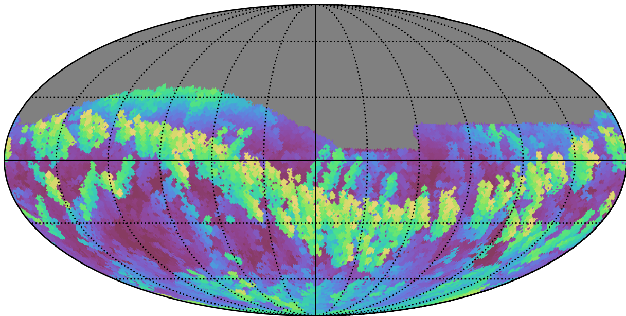
extra_ss_neo2_v3.4_10yrs Yr 1 i band: Max airmass
