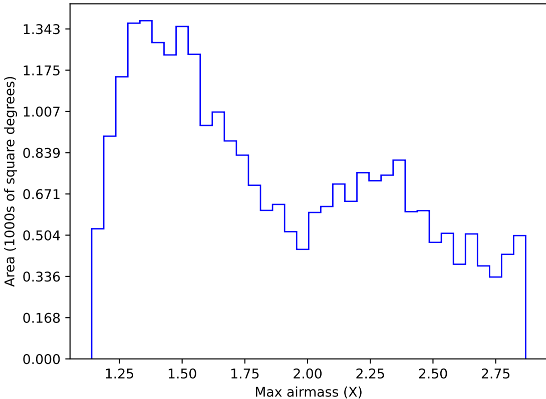
extra_ss_neo2_v3.4_10yrs Yr 1 i band: Max airmass
