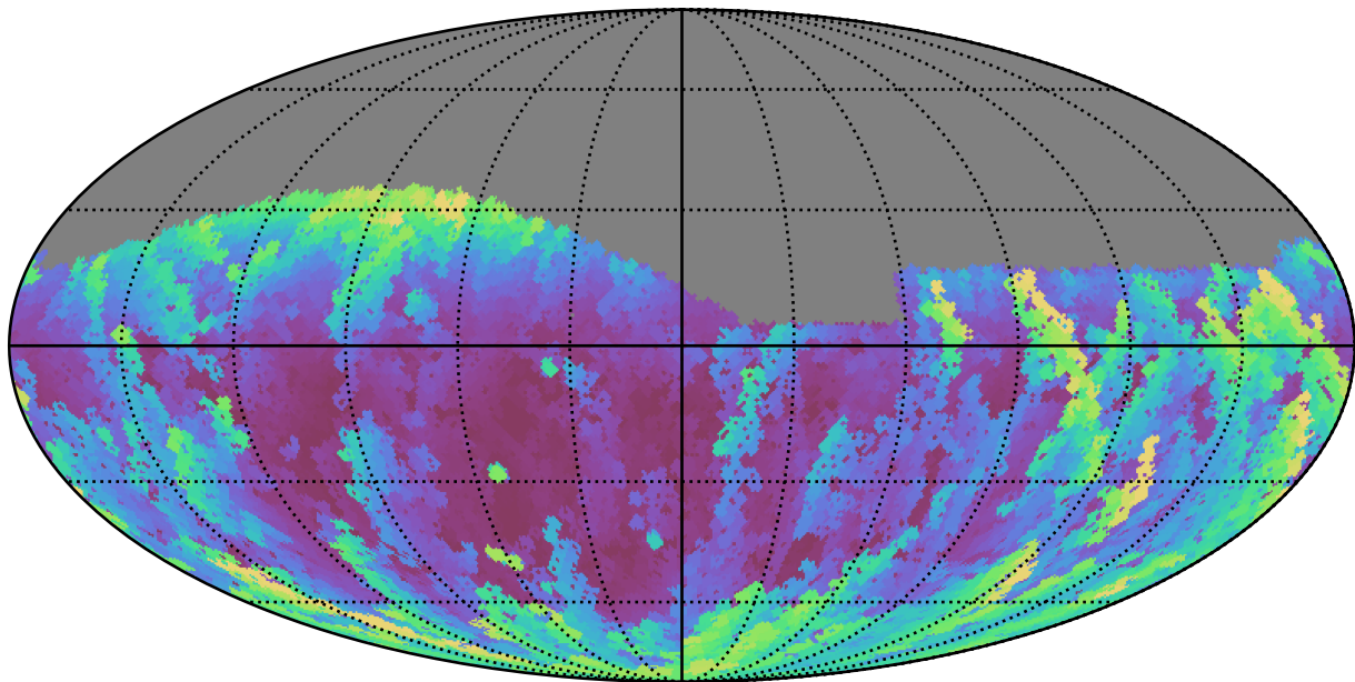
extra_ss_neo2_v3.4_10yrs Yr 1 g band: Max airmass
