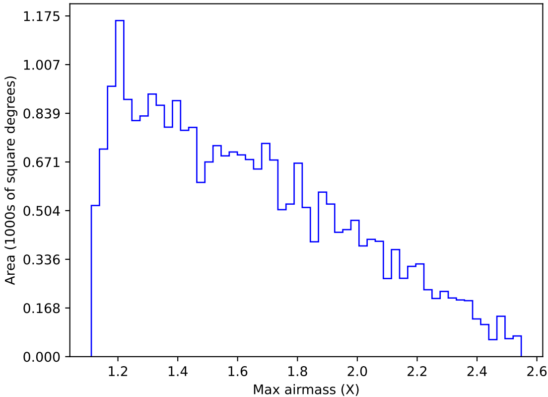
extra_ss_neo2_v3.4_10yrs Yr 1 g band: Max airmass
