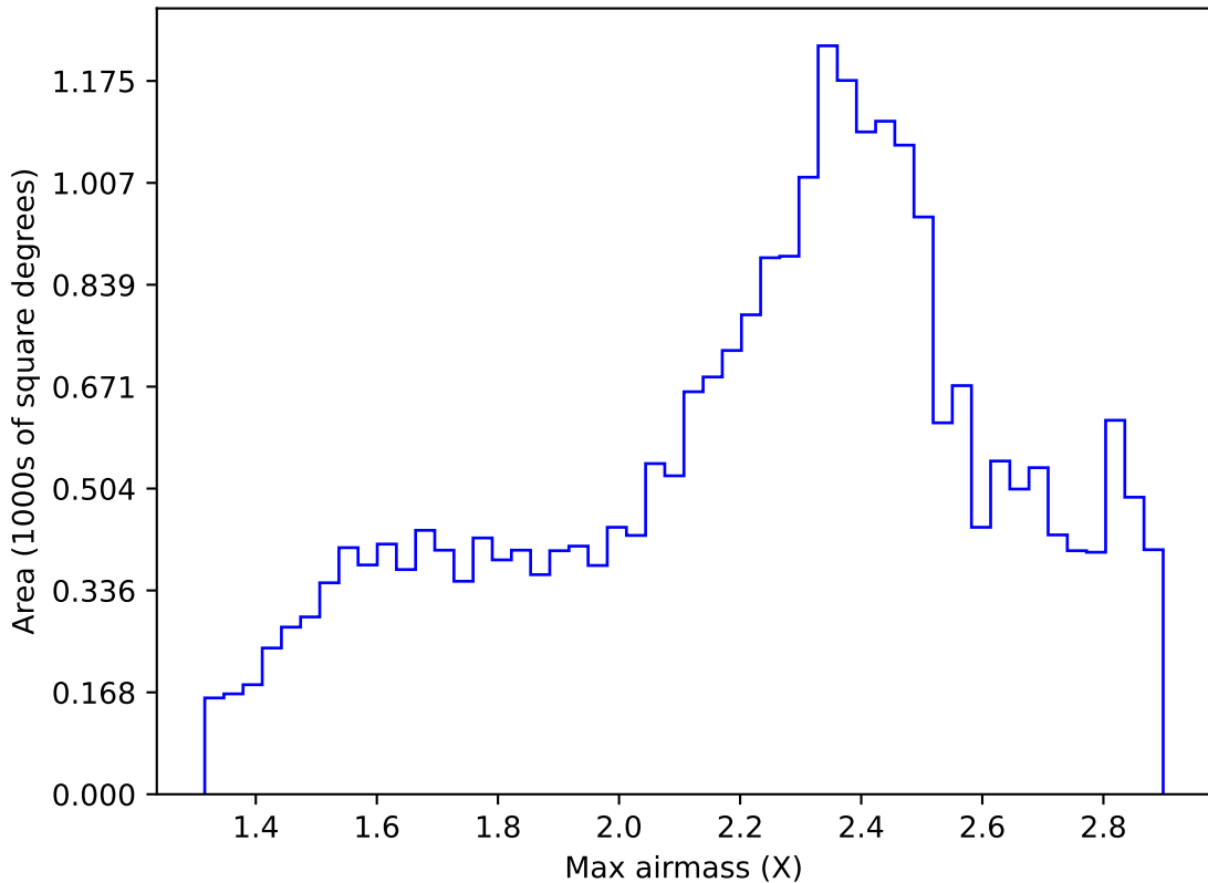
extra_ss_neo2_v3.4_10yrs Yr 1 all bands: Max airmass
