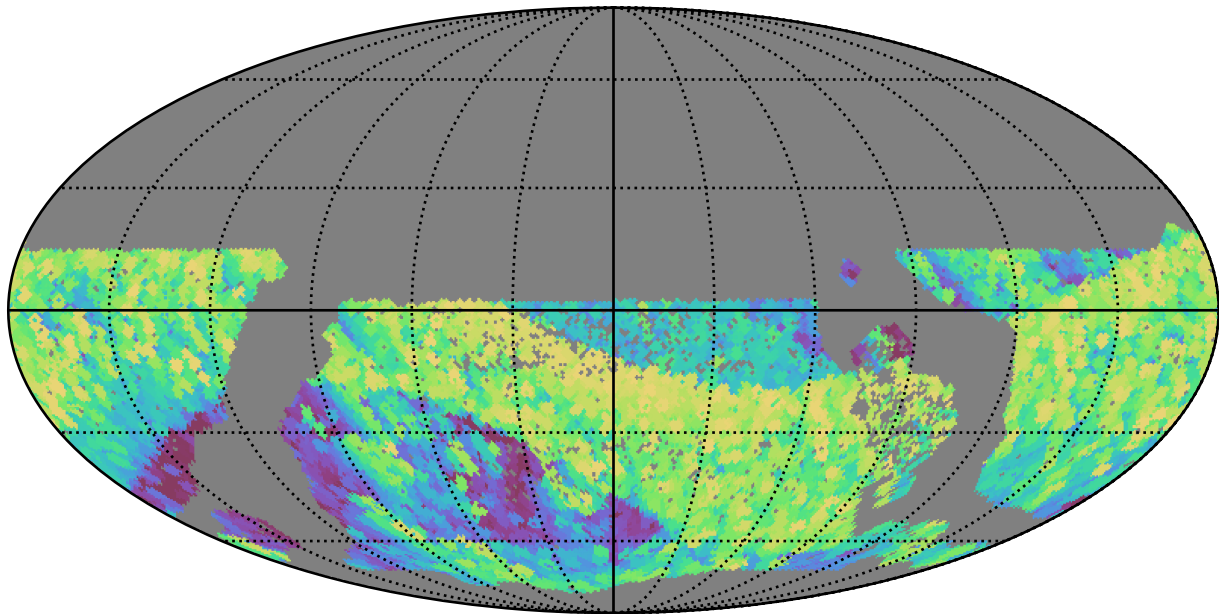
extra_ss_neo2_v3.4_10yrs WFD z band: Max airmass
