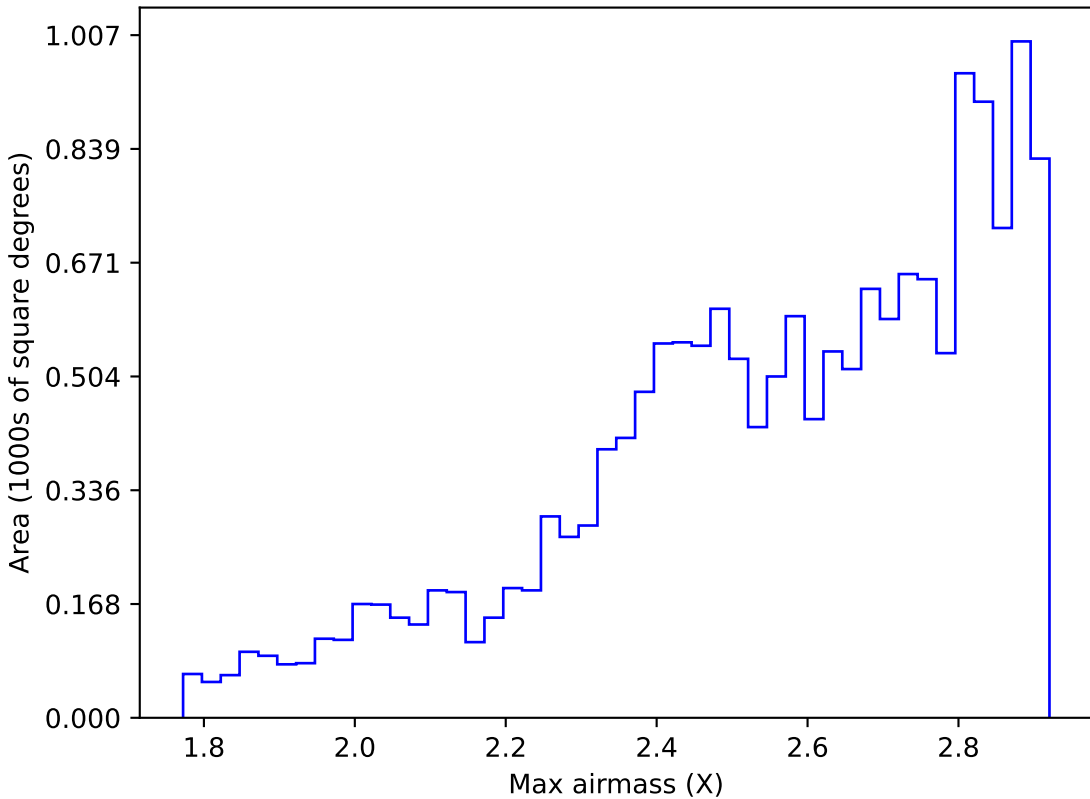
extra_ss_neo2_v3.4_10yrs WFD z band: Max airmass
