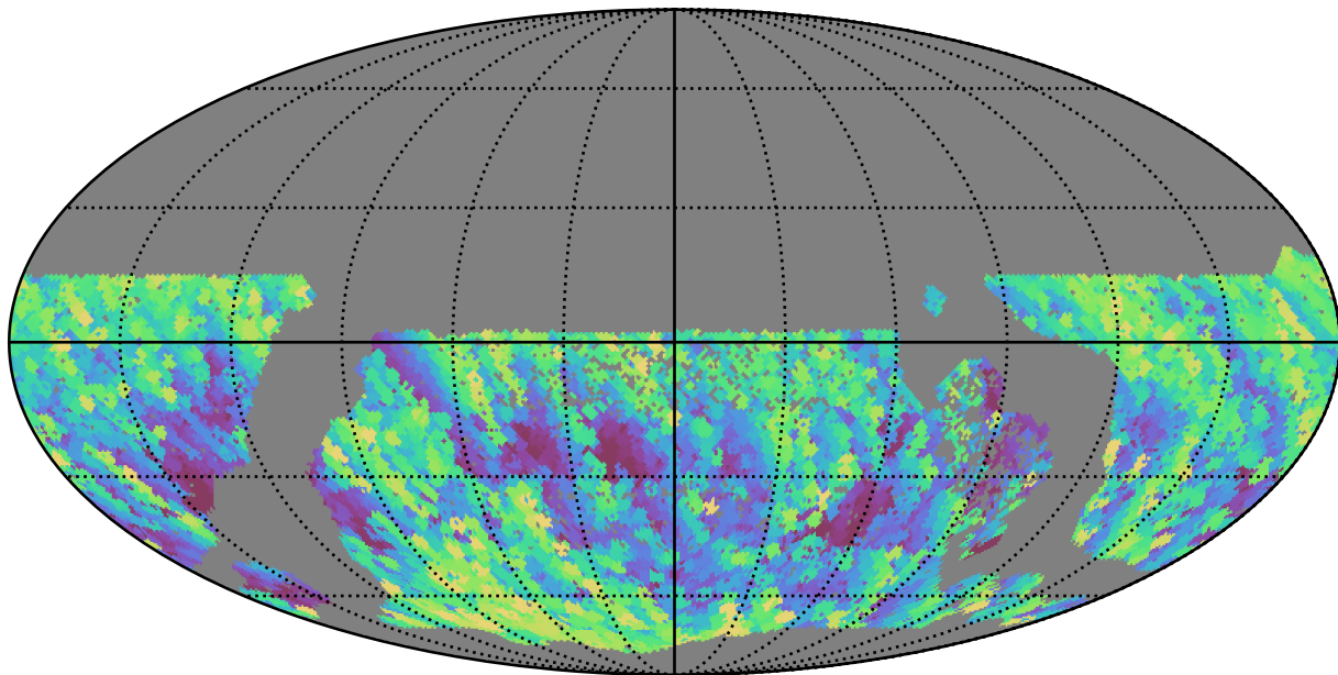
extra_ss_neo2_v3.4_10yrs WFD y band: Max airmass
