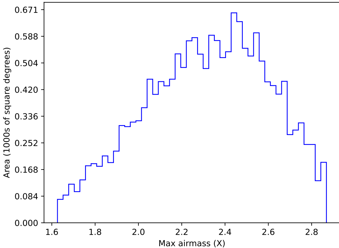
extra_ss_neo2_v3.4_10yrs WFD y band: Max airmass
