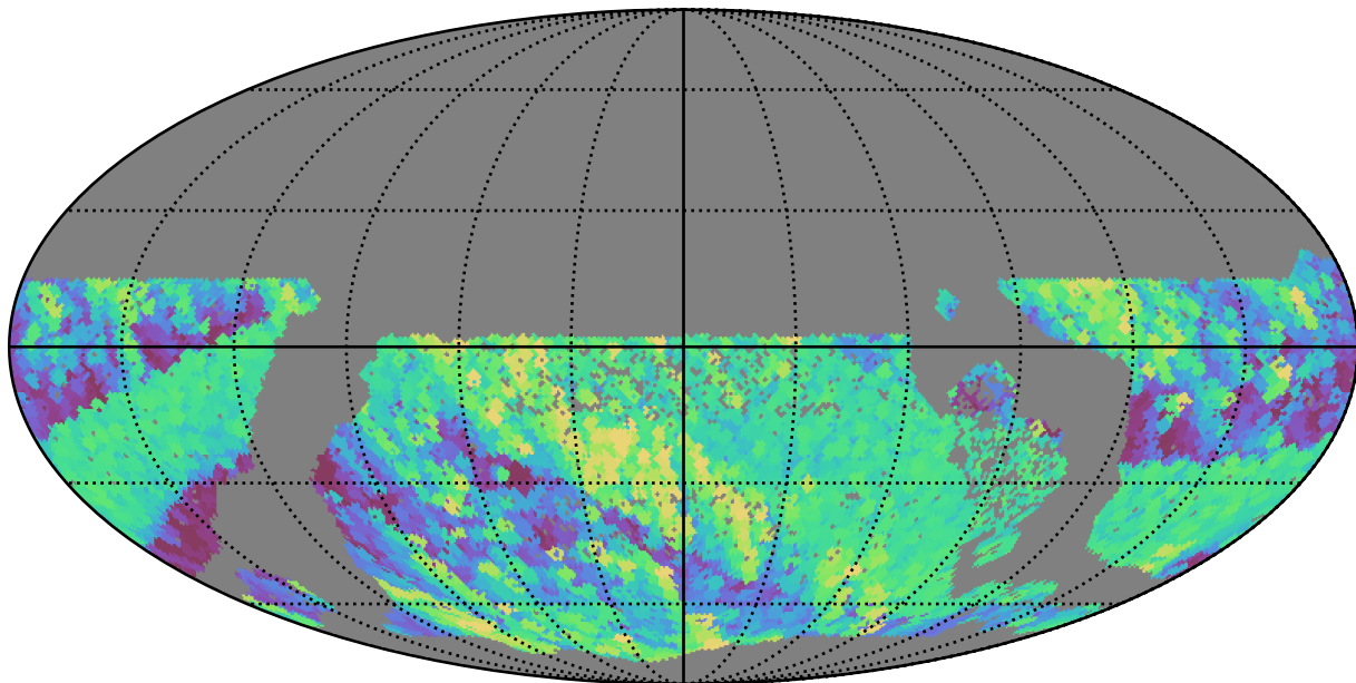
extra_ss_neo2_v3.4_10yrs WFD r band: Max airmass
