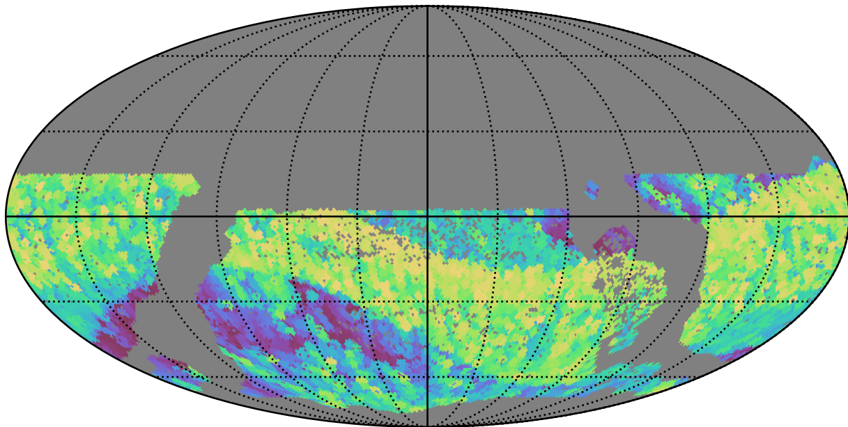
extra_ss_neo2_v3.4_10yrs WFD i band: Max airmass
