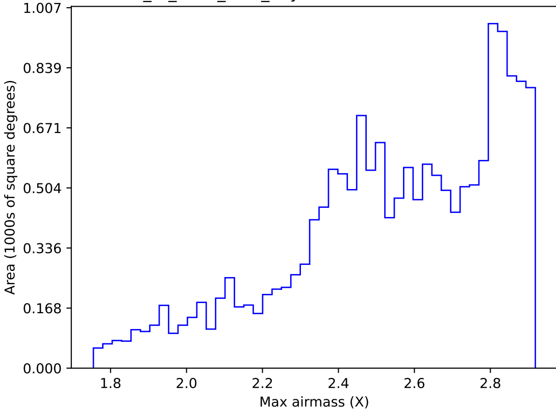
extra_ss_neo2_v3.4_10yrs WFD i band: Max airmass
