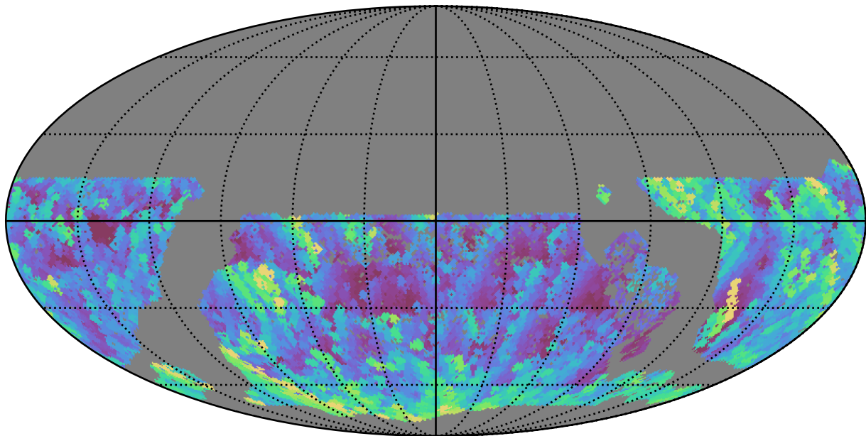
extra_ss_neo2_v3.4_10yrs WFD g band: Max airmass
