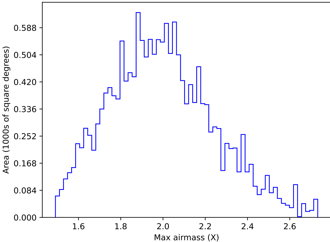
extra_ss_neo2_v3.4_10yrs WFD g band: Max airmass
